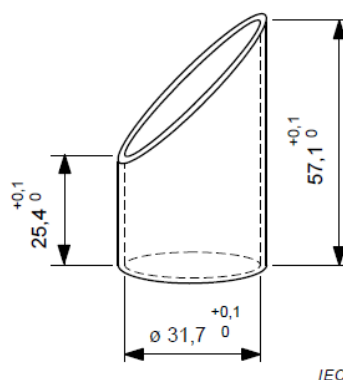
Figure 3 – Ingestion gauge
