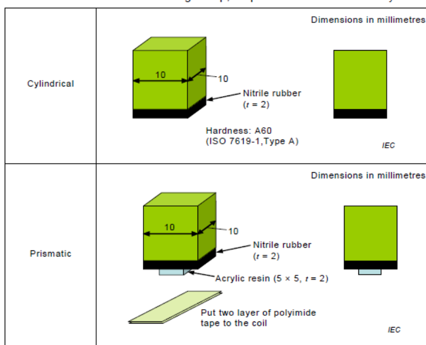
Figure 2 – Jig for pressing
