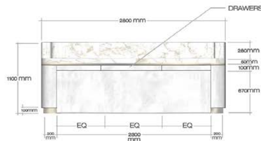
REAR ELEVATION
