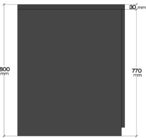
LEFT ELEVATION
