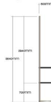
LEFT ELEVATION
