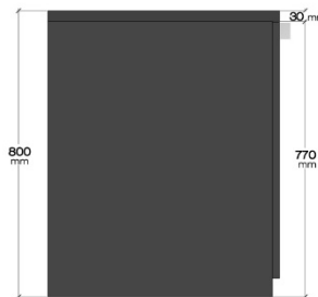
LEFT ELEVATION
