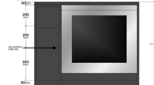
OPEN CABINET
