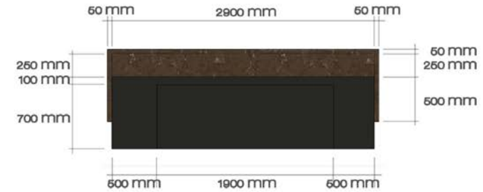
LEFT ELEVATION
