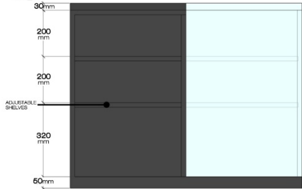
OPEN CABINET
