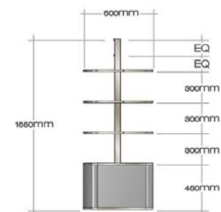
LEFT ELEVATION
