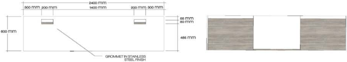
TOP VIEW
