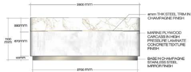
FRONT ELEVATION
