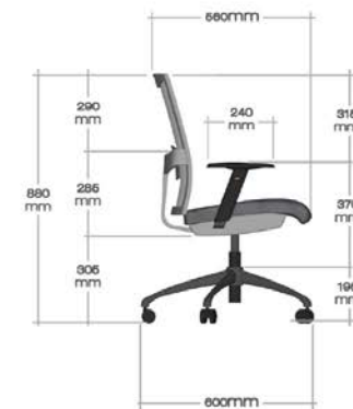
LEFT ELEVATION
