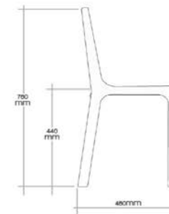
LEFT ELEVATION
