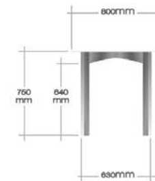
LEFT ELEVATION
