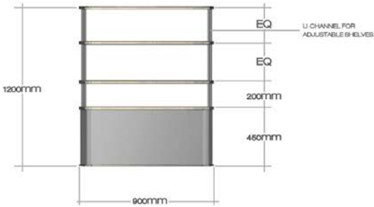
FRONT ELEVATION
